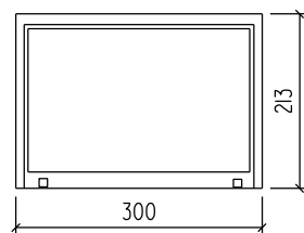
FRONT
